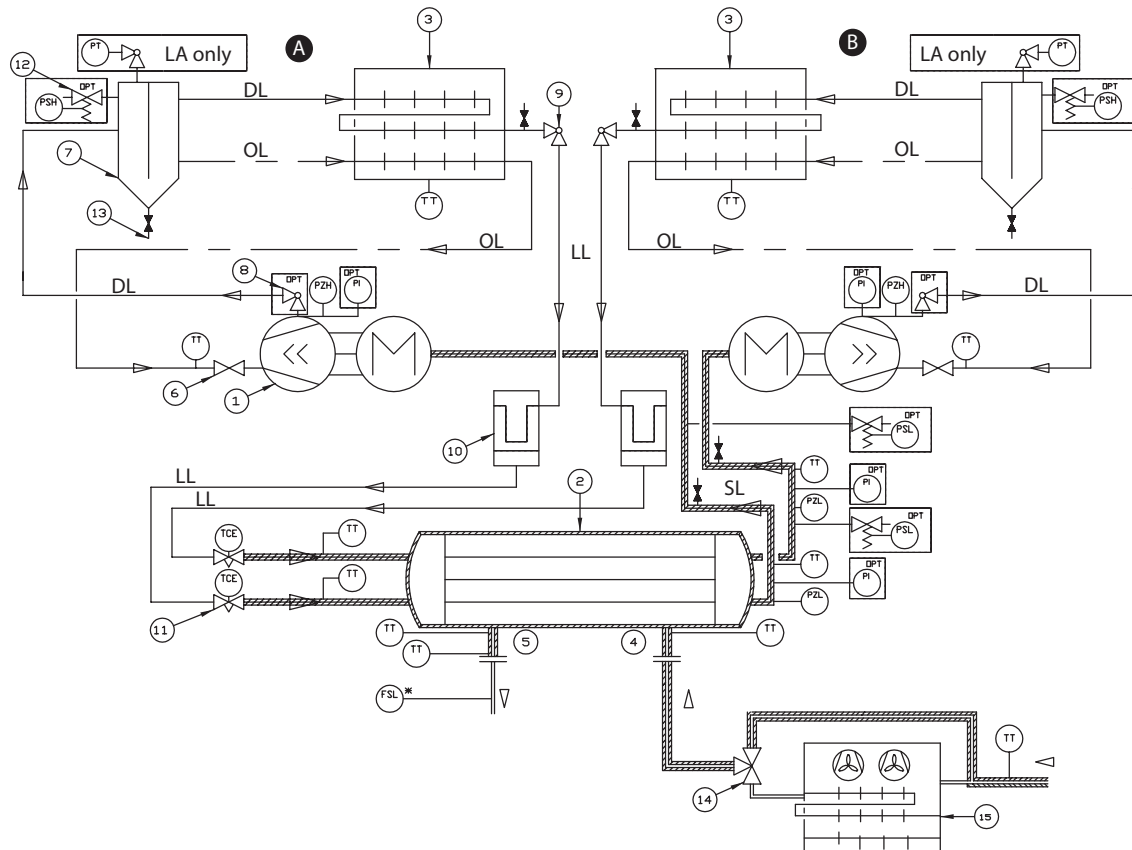
Figure 28 - System schematic for Free-Cooling units
