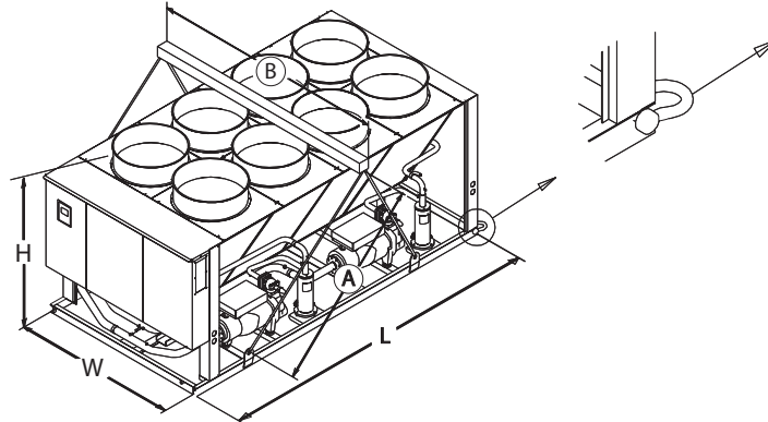
Figure 3 - Rigging the Unit
