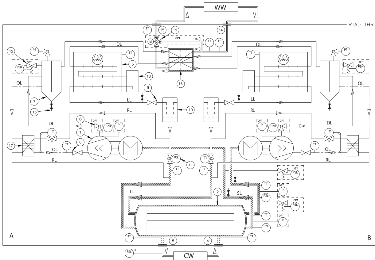
Figure 29 - System schematic for Total Heat Recovery units
