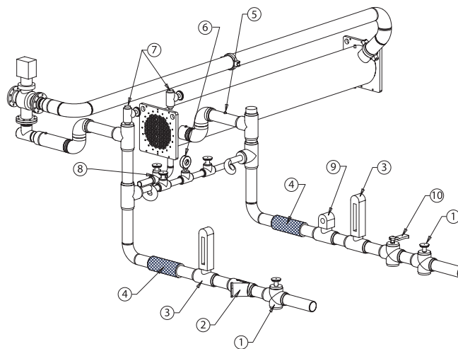
Figure 20 - Suggested piping for typical RTAD Free Cooling evaporator
