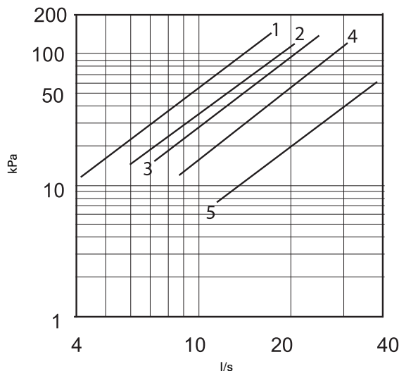
Figure 4 - Evaporator Water Pressure Drop RTAD
