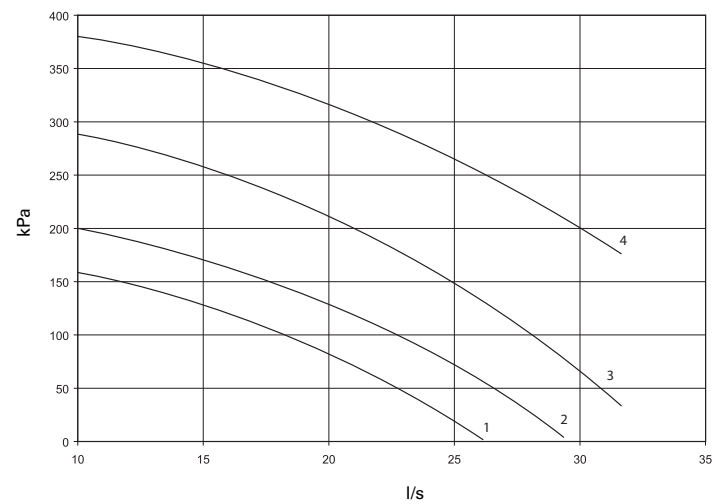
Figure 6 - RTAD 115HE - 125HE - 145SE - 150SE Dual pump available static pressure
