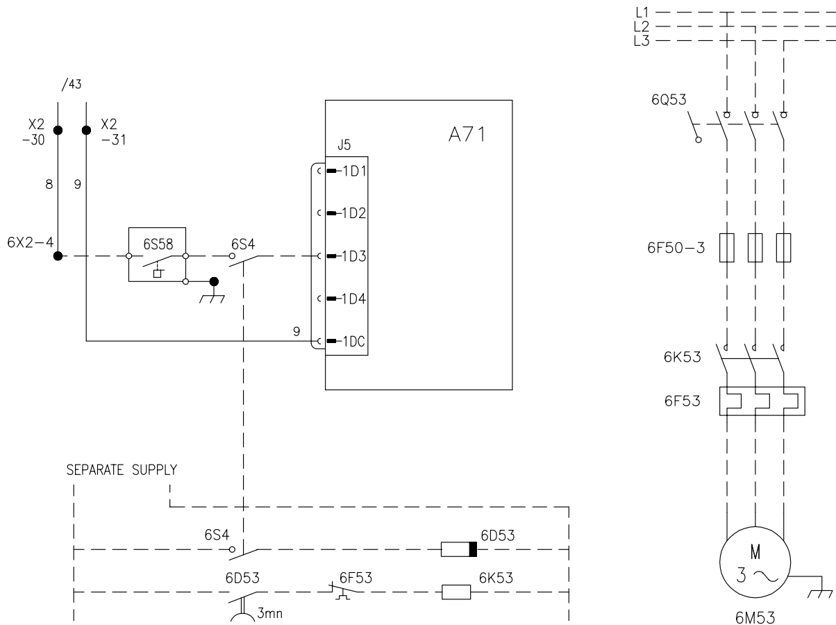
Figure 25 - Control wiring for pump
