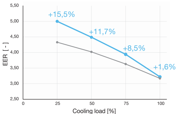
The graph shows the chiller efficiency with the variation of the load rate and air temperature (ESEER operating conditions).
