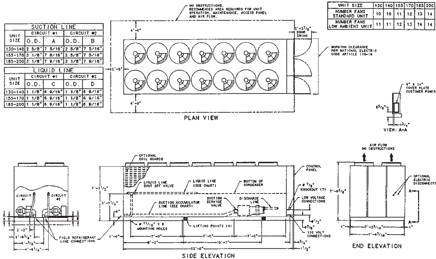
Figure 12 Dimensions and Clearances for RTAA Outdoor Unit with Remote Evaporator Option
