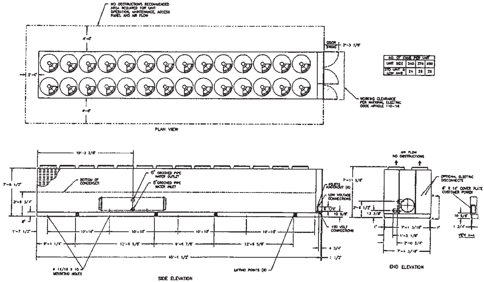
Figure 11 Dimensions and Clearances for RTAA Packaged Unit – 340 to 400 Ton
