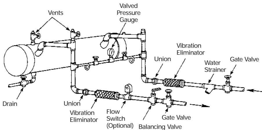
Figure 22 Suggested Piping for Typical RTAA Evaporator
