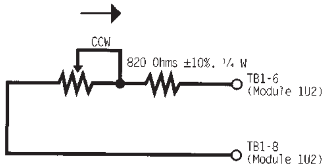
Figure 39 Resistor and Potentiometer Arrangement for External Current Limit Setpoint
