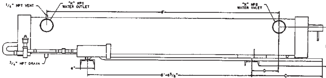
SIDE ELEVATION
