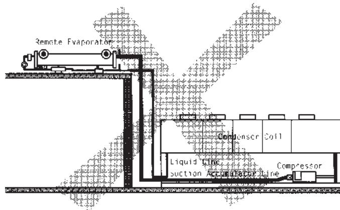
Figure 28 Restricted Installation – Evaporator is on a Higher Plane than the Outdoor Unit
